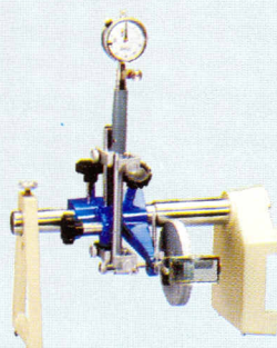
Calibration of Bore Gauge (Vertical)
