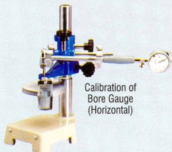
Calibration of Plunger Type Dial Gauge
